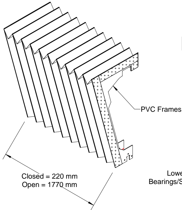
Isometric Front View
